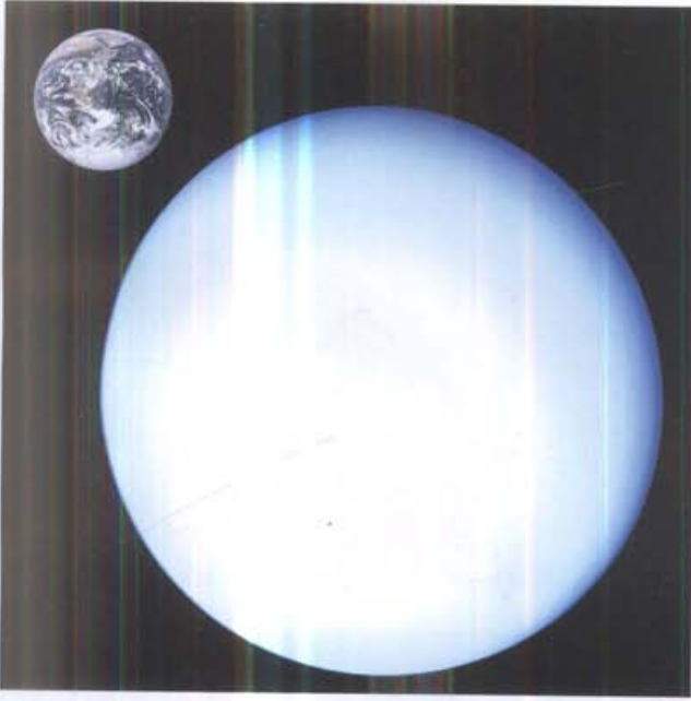
Uranus-earth comparison
