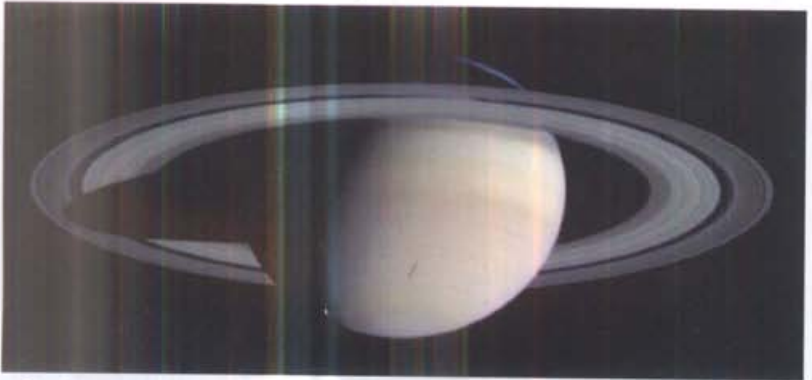
Saturn
